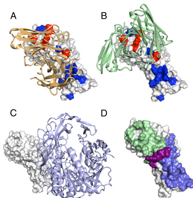
Fig. 3. Computational models of MERS CoV RBD in complex with antibody LCA60. (A and B) Structures of the complex between mAb LCA60 (light green and orange cartoons) and RBD MERS (white surface) obtained by computational docking. S protein mutants that affect (red) or do not affect (blue) antibody binding are shown. Only model B is consistent with the mutation data. (C) Experimental structure of the complex between CD26 (light blue cartoon) and MERS RBD [Protein Data Bank (PDB) ID code 4KR0]. (D) Footprint of LCA60 antibody (light green) and CD26 (light blue) on the surface of MERS RBD (white). Residues in contact with both LCA60 and CD26 are shown in violet.
